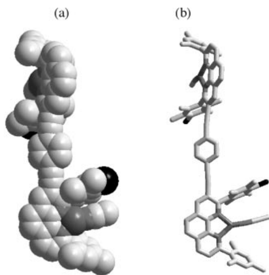
Figure 1. a) Space filling and b) stick representation of the crystal structure of [\text{Cu}_2(\mathbf{2})(\text{MeCN})_2]^{2+} .
