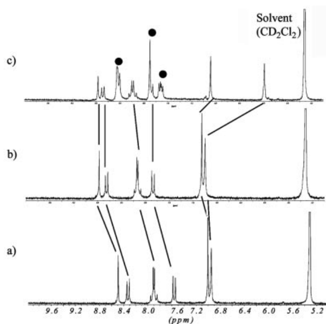
Figure 2. ^1\text{H} NMR changes in the aromatic region of 2 upon complexation with 3a . a) free 2 ; b) [\text{Cu}_2(\mathbf{2})(\text{MeCN})_2]^{2+} ; c) [\text{Cu}_2(\mathbf{2})(\mathbf{3a})_2]^{2+} . Signals in Figure c being marked by filled spheres belong to phenanthroline ( 3a ) protons.
