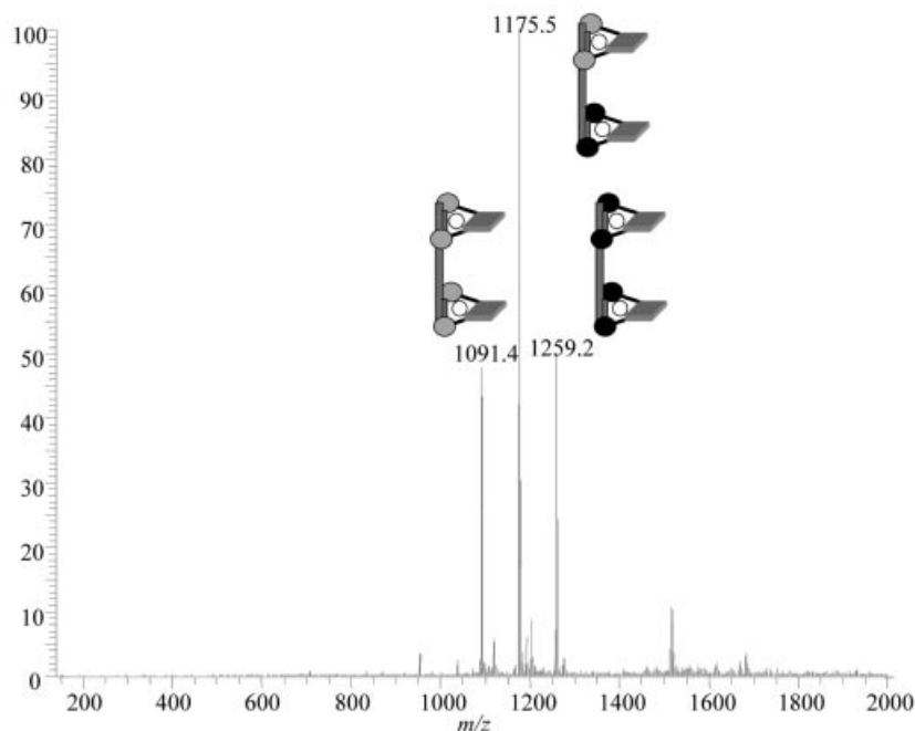
Figure 5. ESI-MS of the reaction mixture obtained when 1a , 4a , 4b are treated with Cu^I salt in dichloromethane.
