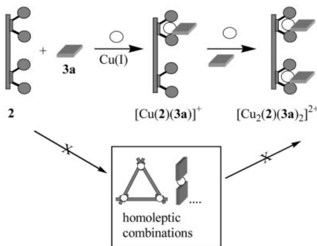
Scheme 4. Self-assembly path for R1 .
