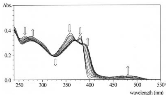
Figure 3. Spectrophotometric titration of 2 and 1,10-phenanthroline ( 3a ) by aliquot amounts of \text{Cu}^{\text{I}} salt in 20 additions. Solvent: dichloromethane. T = 25(1)^\circ\text{C} . [\mathbf{2}] = 1.20 \times 10^{-6} \text{ M} and [\mathbf{3a}] = 2.40 \times 10^{-6} \text{ M} .
